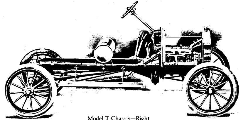
Model T Chassis—Right
