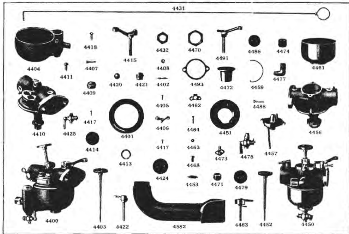
Plate No. 14—1913 Kingdon and Holley Carburetor Parts
