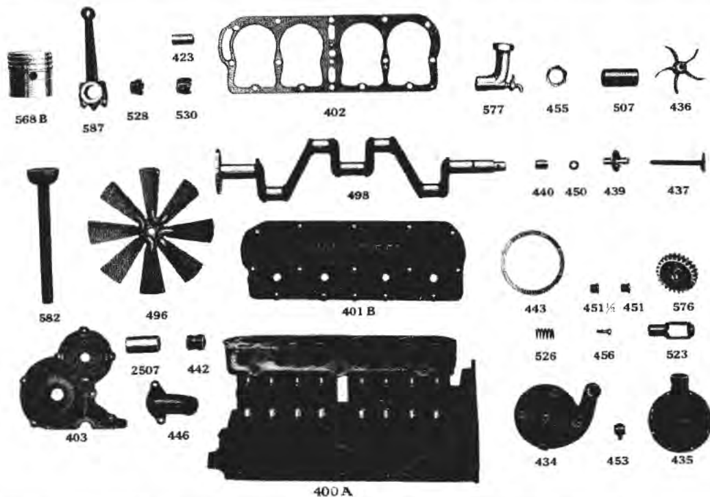
Plate No. 31—Old Style Motor Parts
