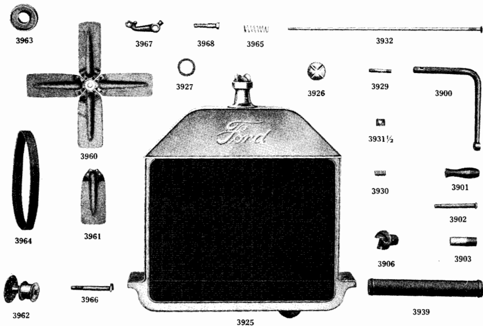
Plate No. 12—Radiator Parts
