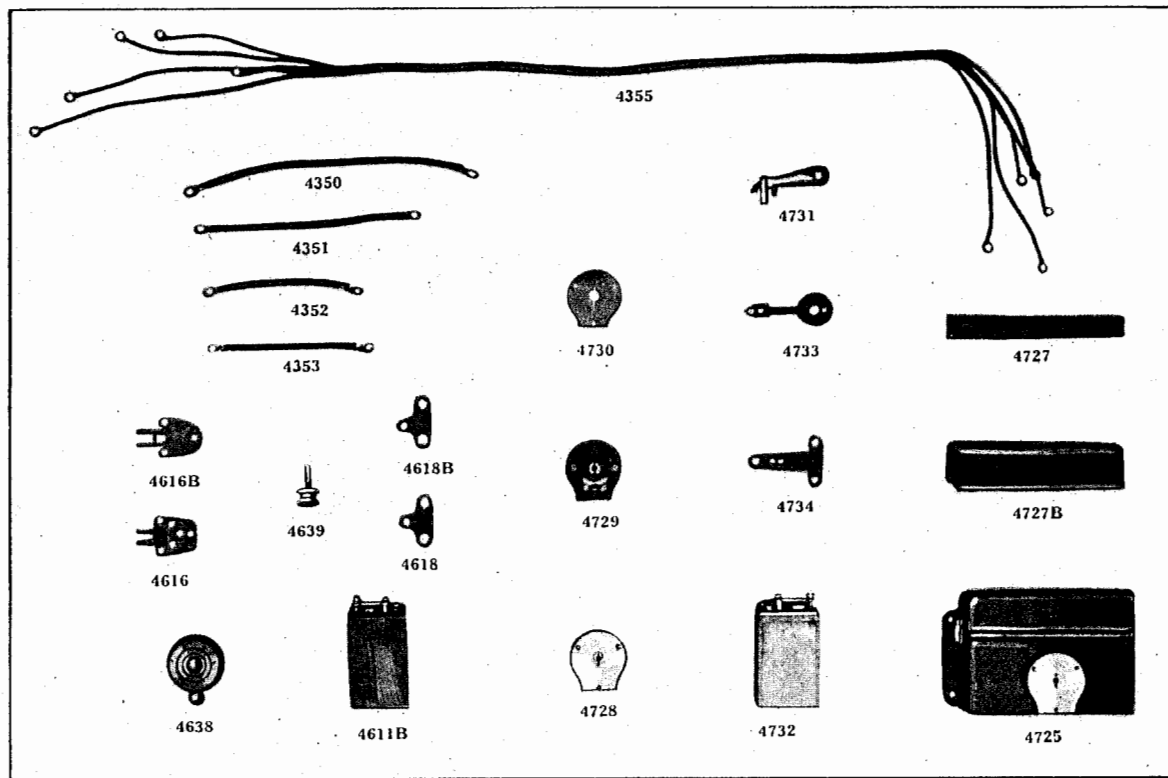
Plate No. 15—Coil Parts and Wiring
