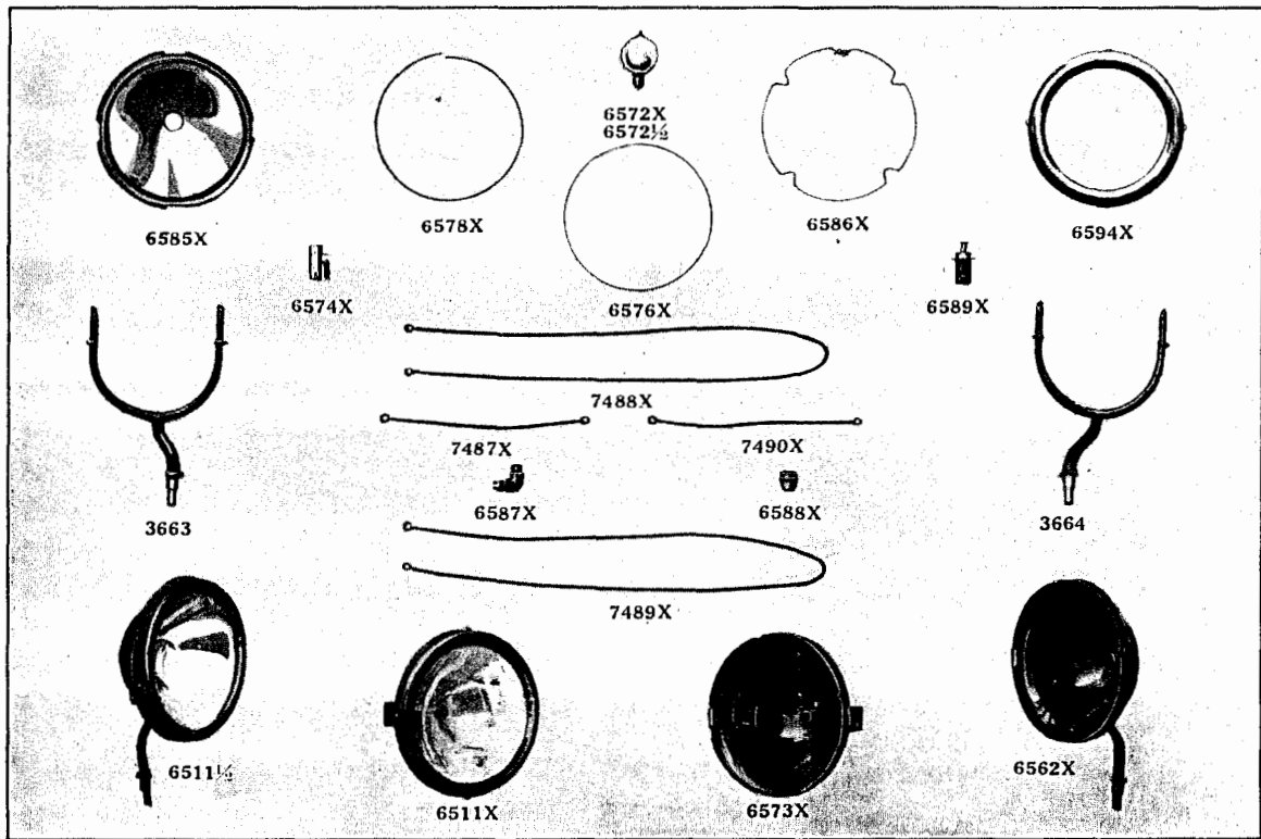
Plate No. 18—1915-17 Electric Head Lamps and Parts
