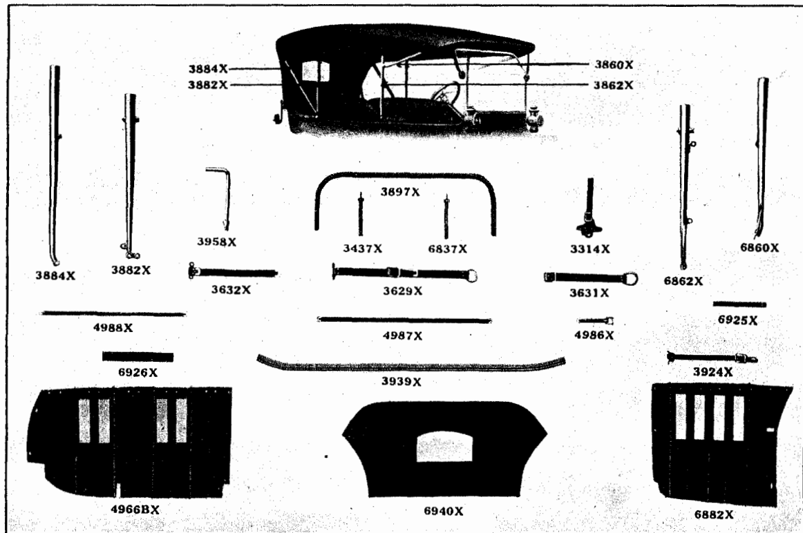
Plate No. 21—1915-17 Touring Car Top and Parts
