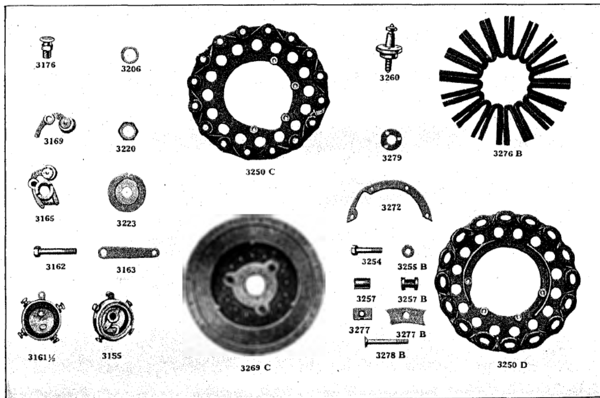
Plate No. 7—Commutator and Magneto Parts
