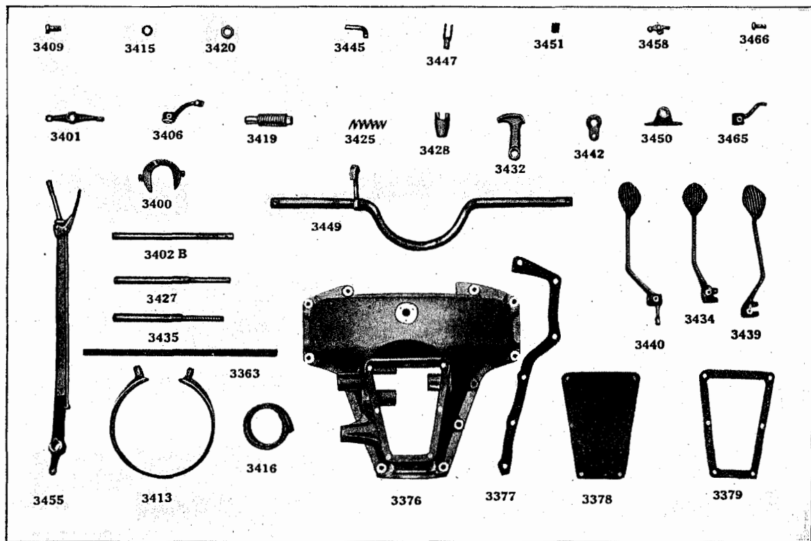
Plate No. 9—Transmission Cover and Control Parts
