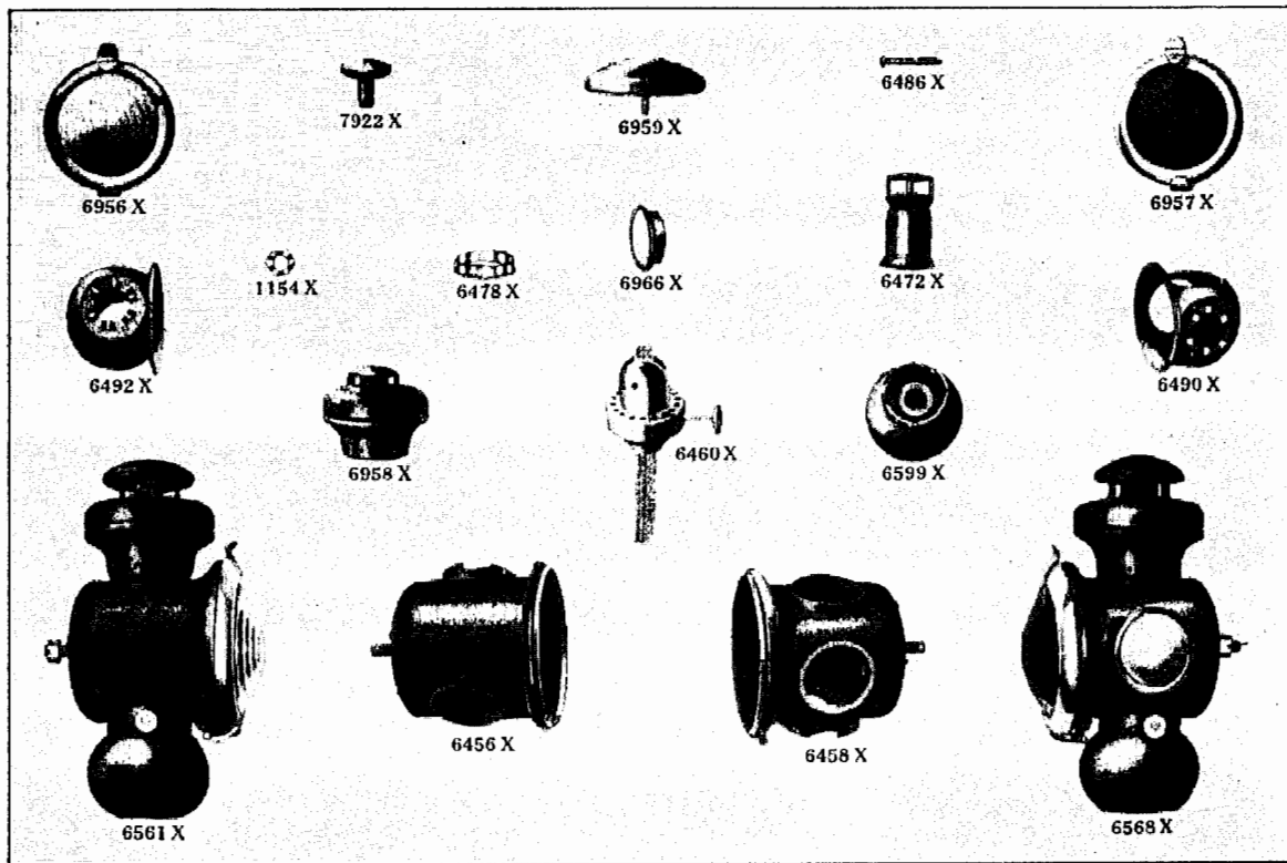
Plate No. 19 - 1915-17 Side and Tail Lamps and Parts
