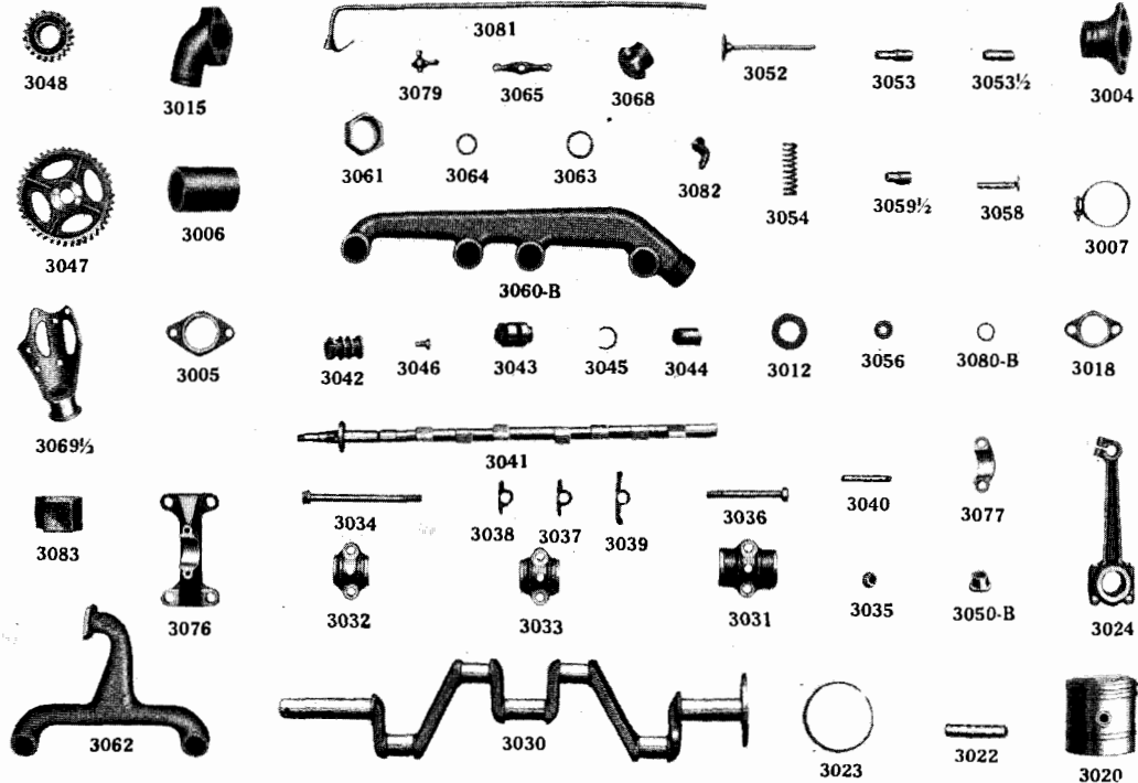
Plate No. 6—Motor Parts
