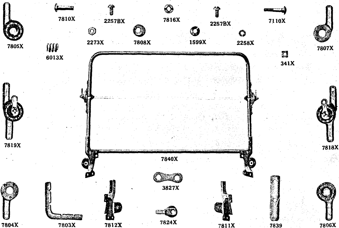
Plate No. 20—1915-17 Windshield and Parts
