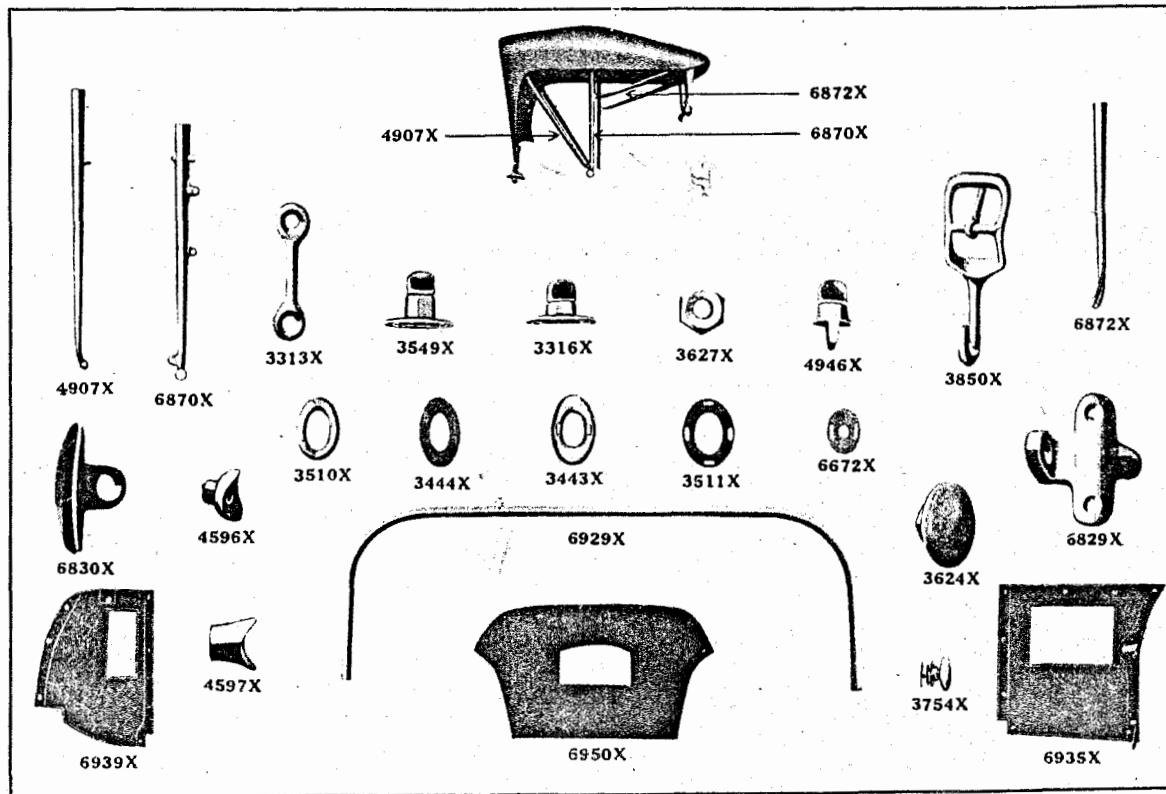
Plate No. 22—1915-1917 Torpedo Car Top and Parts
