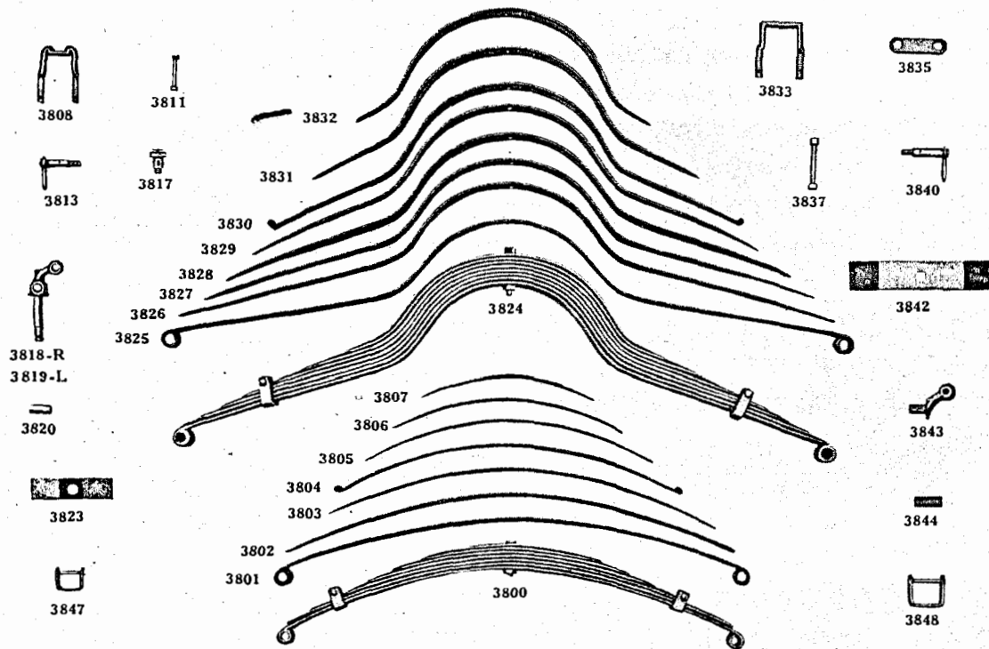
Plate No. II—Spring Parts
