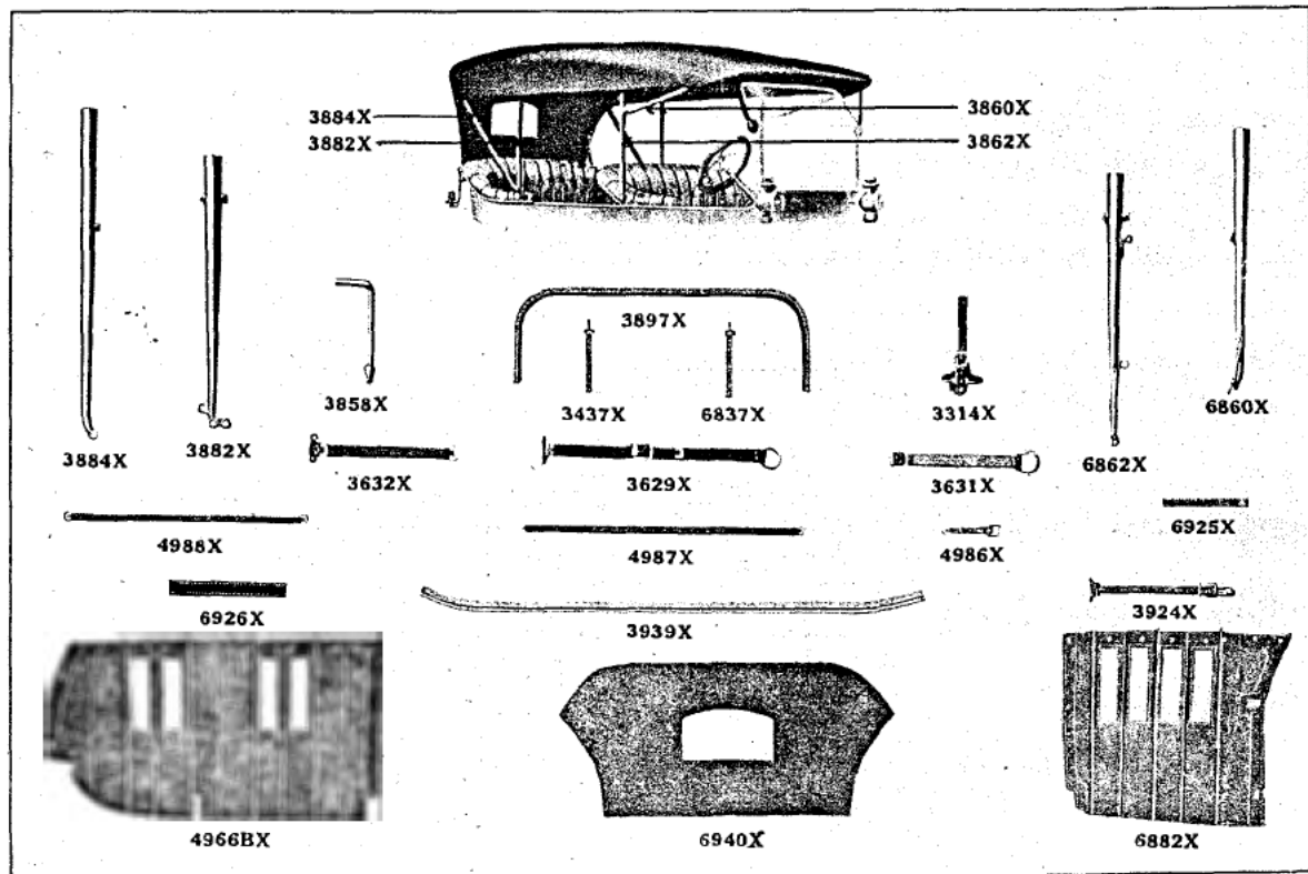
Plate No. 21—1915-1917 Touring Car Top and Parts
