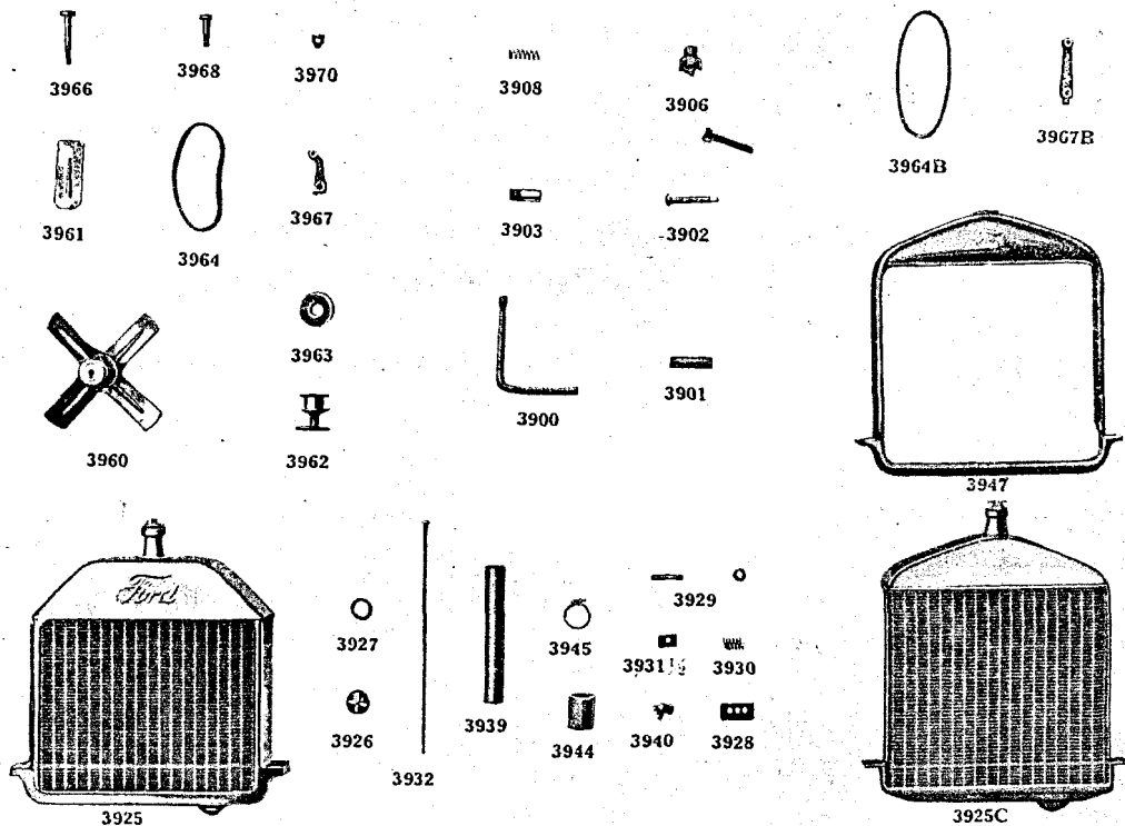
Plate No. 12—Radiator, Fan and Starting Crank Parts
