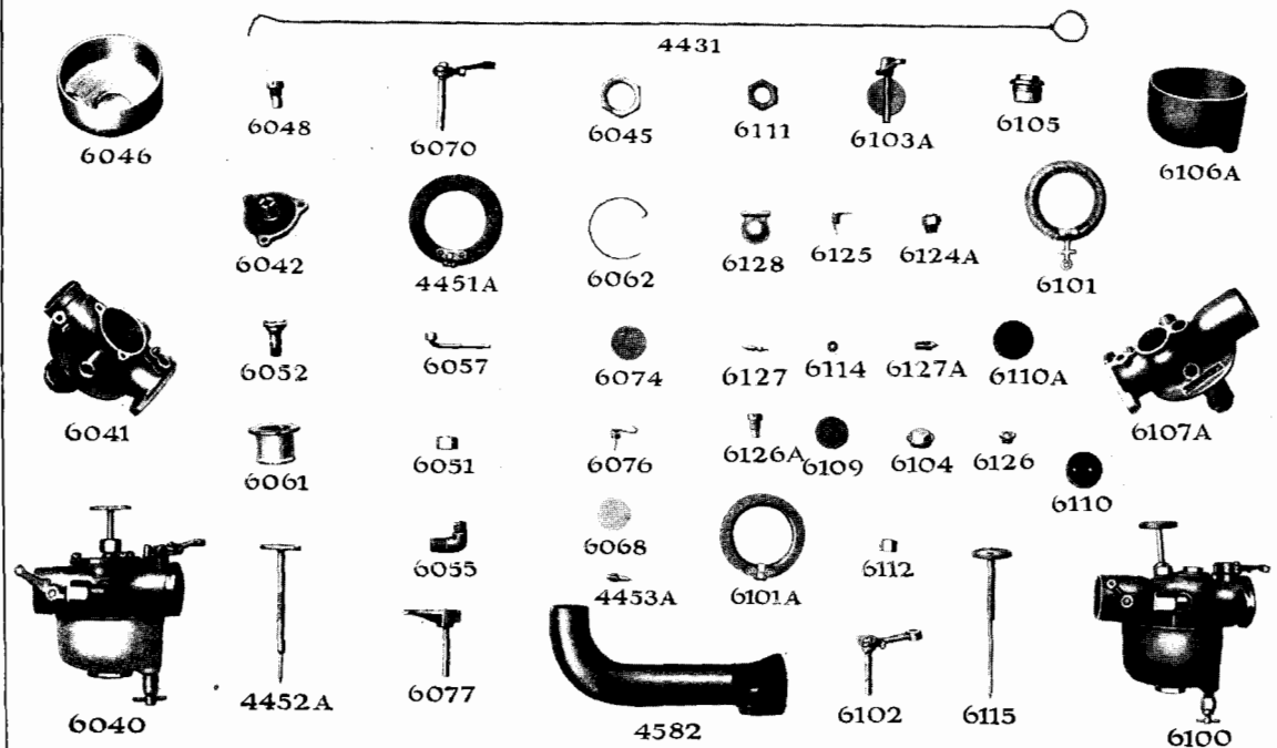
Plate No. 14—Kingston and Holley Carburetor Parts
